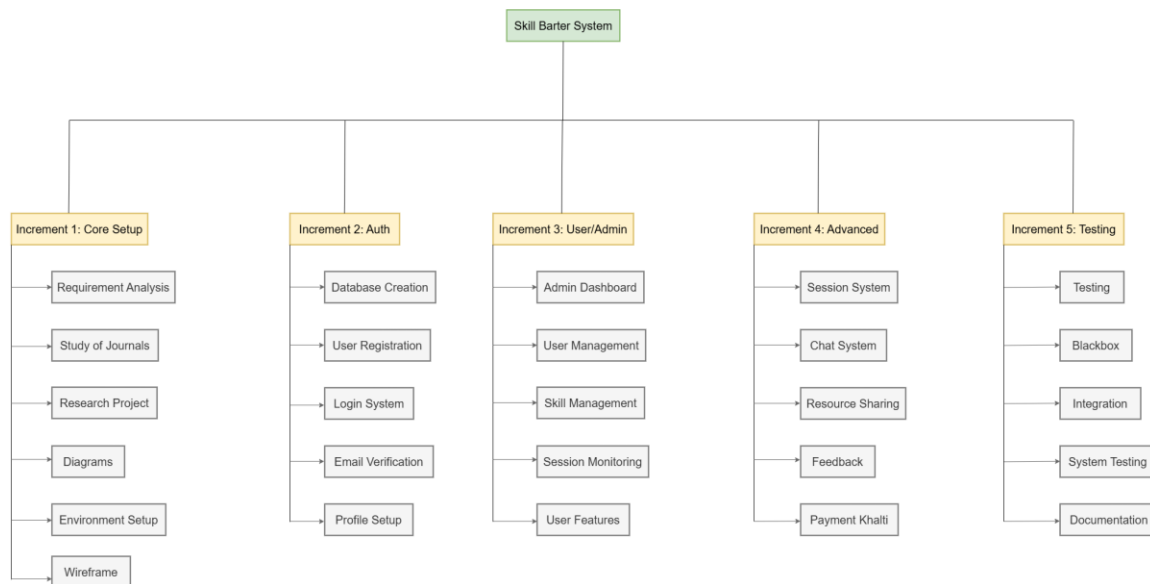
Figure 1: WBS
